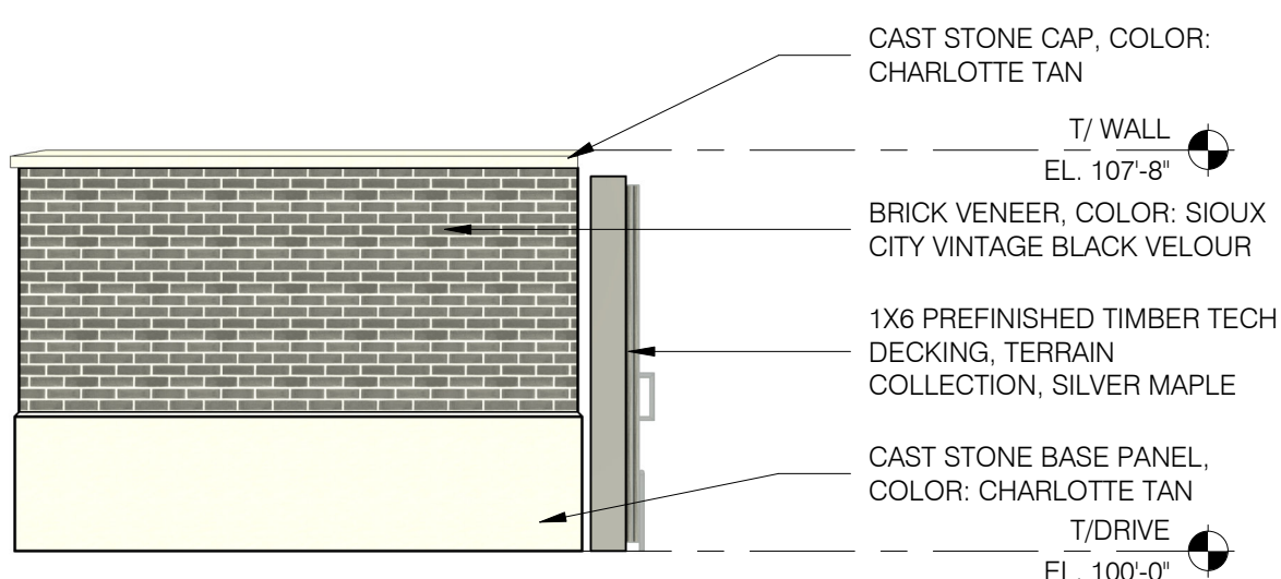
6 SIDE DUMPSTER ELEVATION SCALE: 1/4" = 1'-0"
